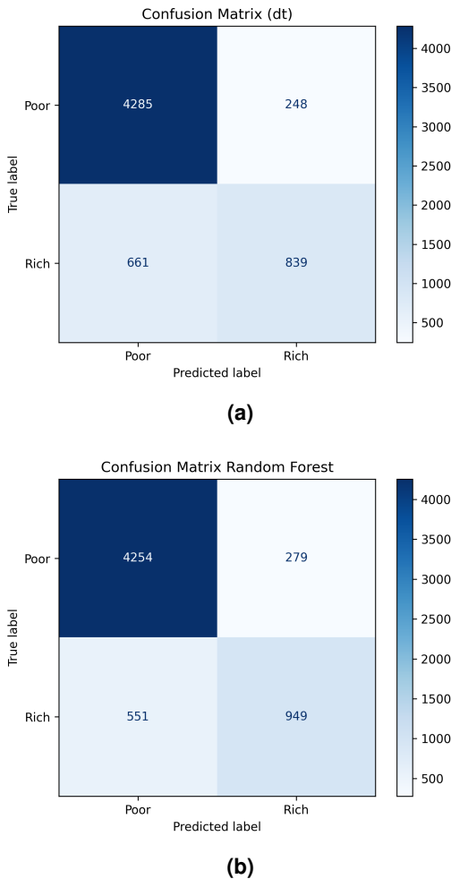
Figure 1. The confusion matrices of the Decision Tree model and the Random Forest model on the test data.
